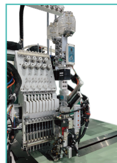
2色散珠装置 2-Color Bead Dispenser Device
